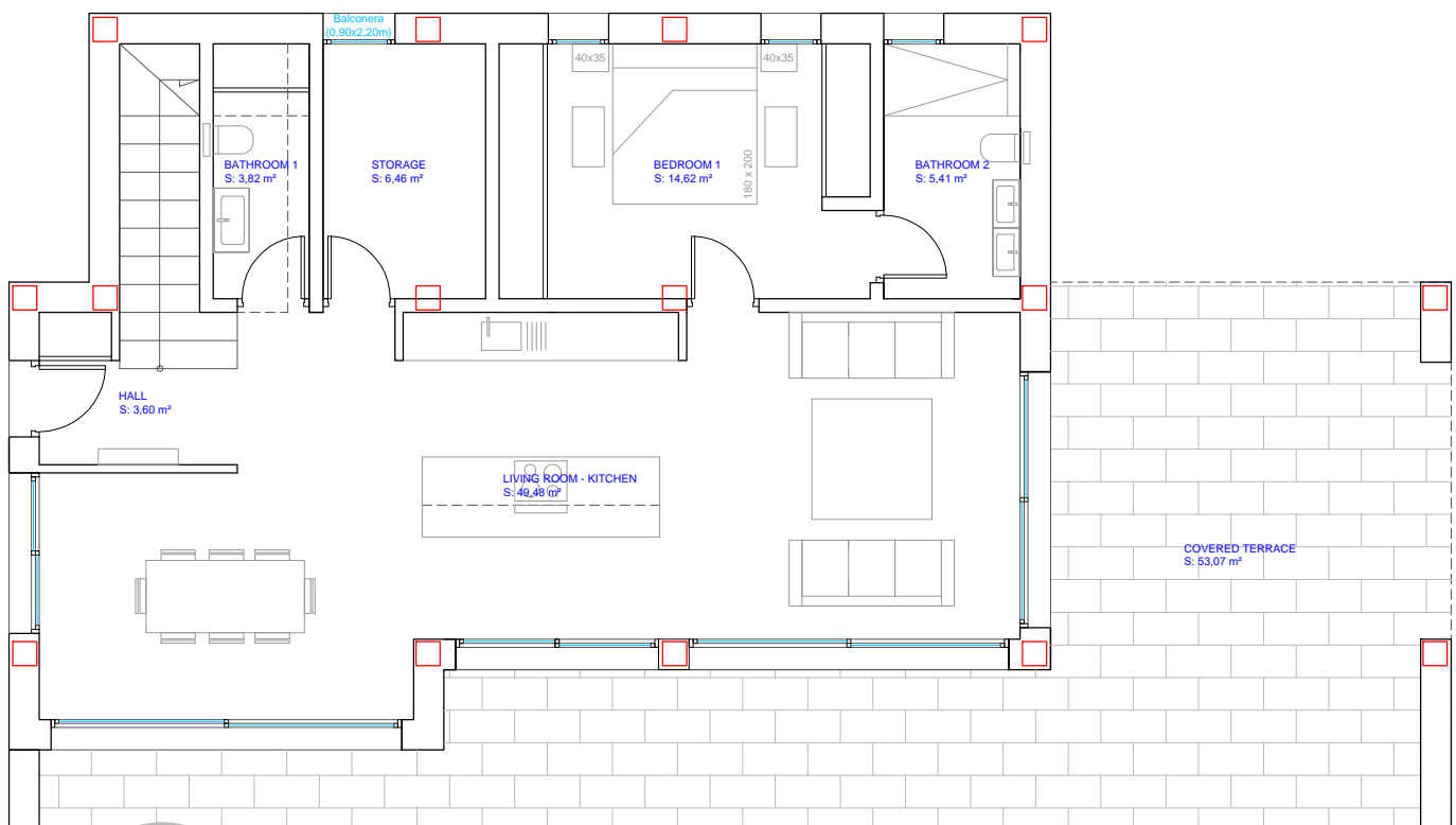
FIRST FLOOR 97,17 m 2
